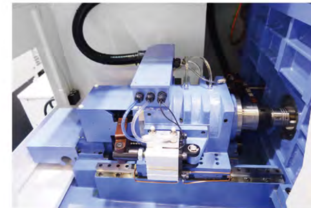
Built-in electro-spindle
